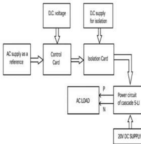
a) Block schematic for a five-level inverter
